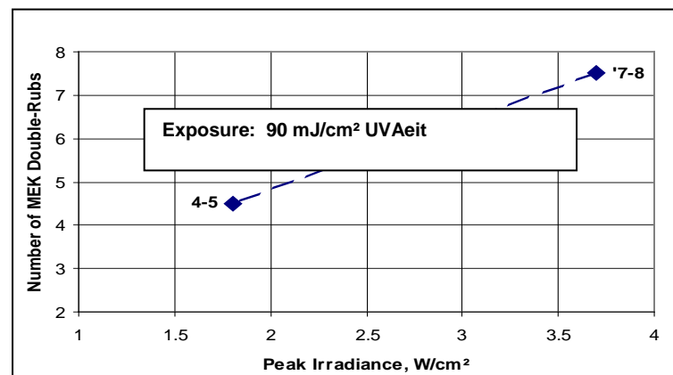
Figure 3 Equivalent exposure at different irradiance of a black ink-jet ink does not yield the same chemical resistance, measured by MEK double-rubs
