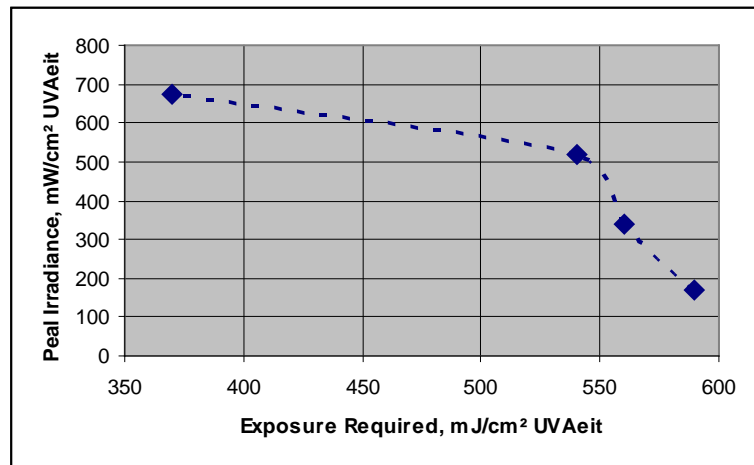
Figure 2 Exposure at different irradiance required to achieve the same cure as determined by adhesion of a 0.7 mil black screen ink to polycarbonate
