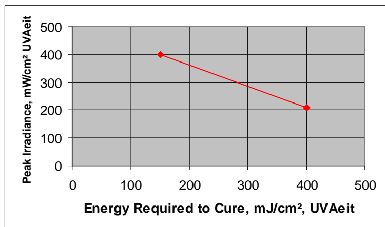
Figure 1. Exposure ( \text{mJ}/\text{cm}^2 ) at different irradiance required to achieve the same chemical resistance (MEK Rubs) at different peak irradiance levels of a clear wood coating
