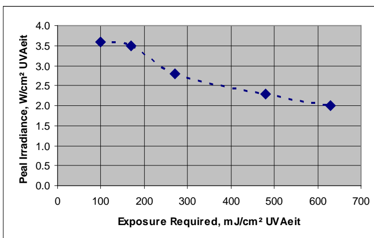
Figure 6 Exposure required to achieve adhesion of a black screen ink on polycarbonate, with the low-irradiance "tails" of the irradiance profile removed
