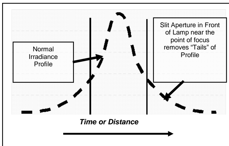
Figure 5 Experimental use of a "slit aperture" to study the peak-to-energy response of a coating
