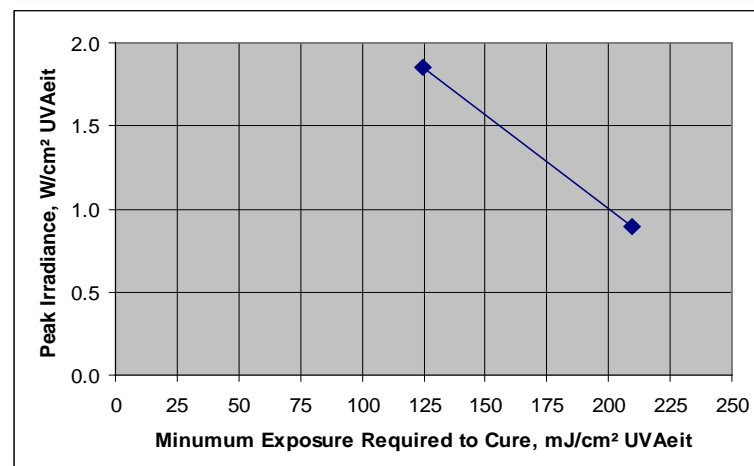
Figure 4 Exposure at different irradiance required to achieve cross-hatch adhesion of a clear hardcoat
