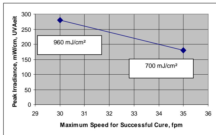
Figure 7 A Thick, Elastomeric Film Can Benefit from Longer, Lower Irradiance Exposure
